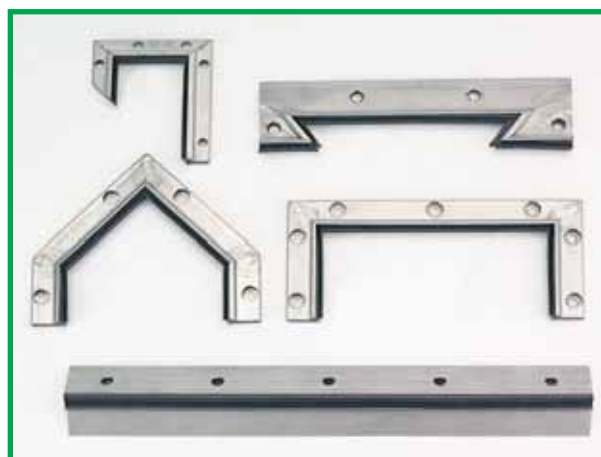
Individual designed wiper according to customer's requirements
