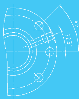
Drilling diagram 1
