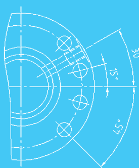
Drilling diagram 2
