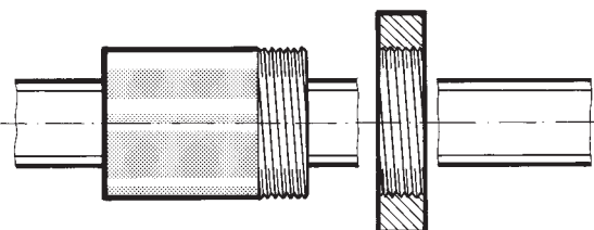
Single nut with and without screw flange
