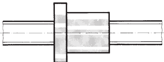
Flanged single nut or internally pre-loaded flanged single nut
